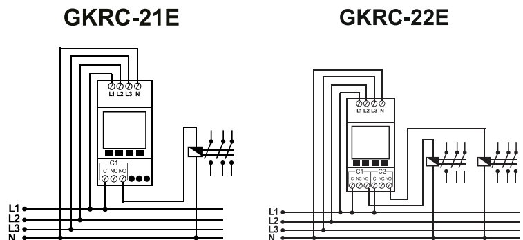
Connection Diagram
