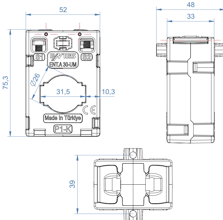
Dimensions (mm)
